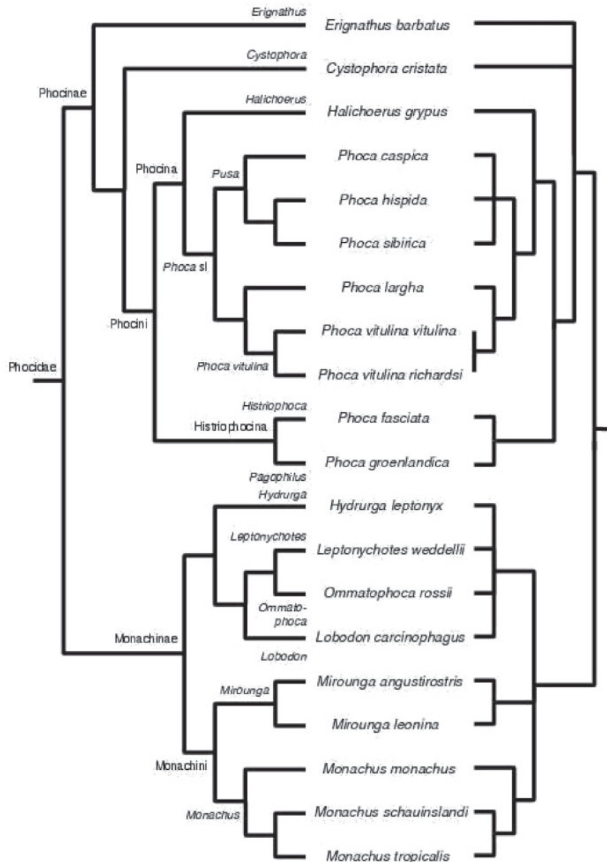
FIGURE 8. The resulting MLS (left) and MRP (right) supertrees for the Phocidae data set obtained from a subset of the source trees used to build the phocid supertree of the carnivore supertree (Bininda-Emonds et al. 1999).
