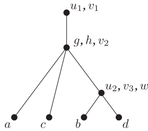
FIGURE 7. The rooted semilabeled tree returned by FREE in the running example when applied to the weighted-descendancy graph shown in Figure 5.
