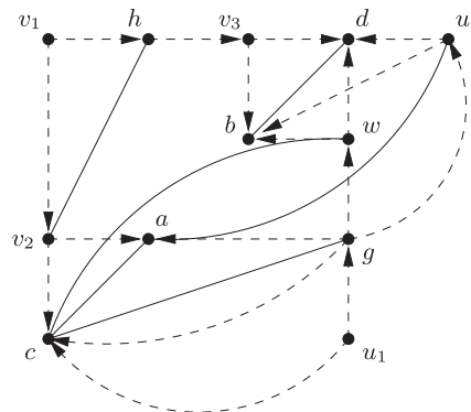
FIGURE 4. The descendancy graph of the collection \mathcal{P}' shown in Figure 3. Arcs are shown as dashed lines with an arrow showing the direction of the arc, while edges are shown as solid lines.
