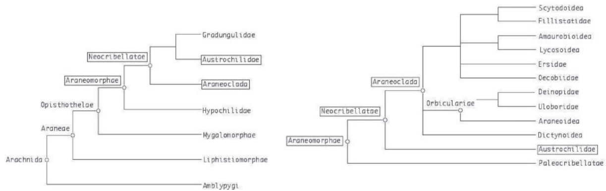
FIGURE 1. Two trees for spiders and related taxa. Internal nodes labeled by higher level taxa (in comparison to the labels at the tips) are indicated with a circle, while taxa common to both trees are enclosed in boxes. These 2 trees, taken from Page (2004), were originally obtained from study S1x6x97c14c42c30 in TreeBASE ( http://www.treebase.org ).
