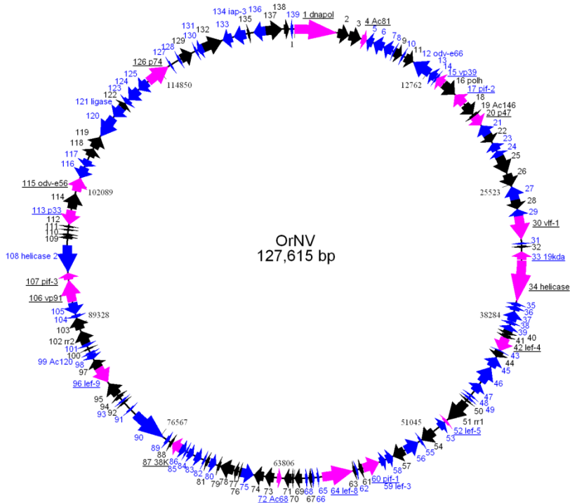
Fig. 1. The genome map of OrNV. ORFs and their transcriptional directions are indicated in arrows. Black color, clockwise coding; blue color, counterclockwise coding; pink color, the 20 baculovirus core gene homologues.
