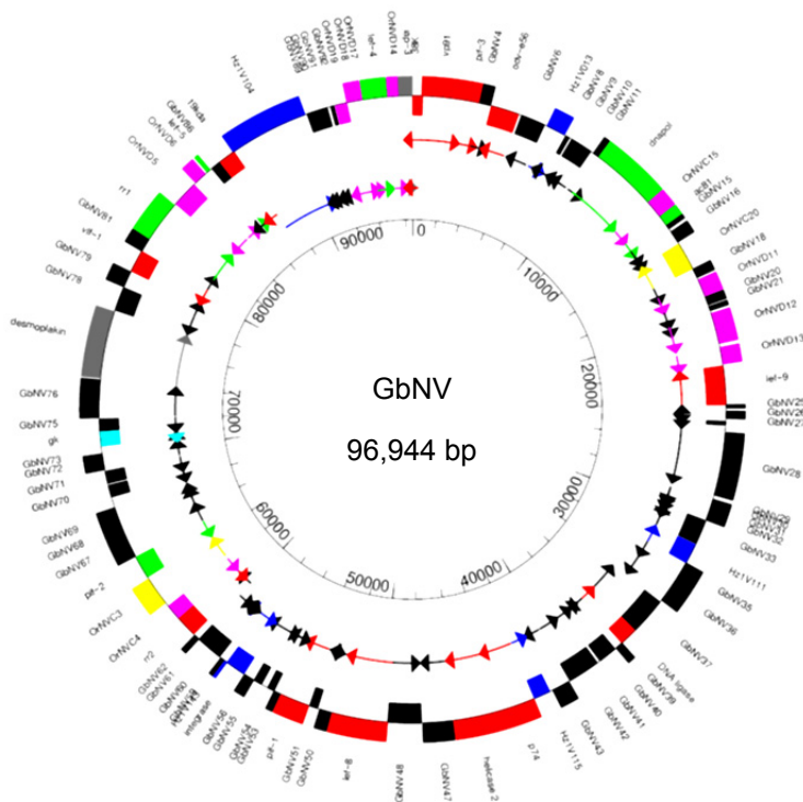
Fig. 2. Circular map of the GbNV genome. ORFs and their transcriptional directions are indicated in boxes and arrows, respectively. Red color, baculovirus and HzNV-1 homologues; black color, GbNV specific ORFs; blue color, HzNV-1 homologues; green color, baculovirus, HzNV-1 and OrNV homologues; pink color, OrNV homologues; yellow color, HzNV-1 and OrNV homologues; light blue, cellular homologues; grey color, baculovirus homologues. Taken from Wang et al. (2007b) with permission from the American Society for Microbiology.
