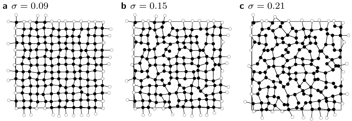
Figure 2. (a–c) Examples of proximity graphs (more precisely, RNG) for different values of \sigma . Connections which cross a periodic boundary are indicated by edges which connect a black node to a white node.
