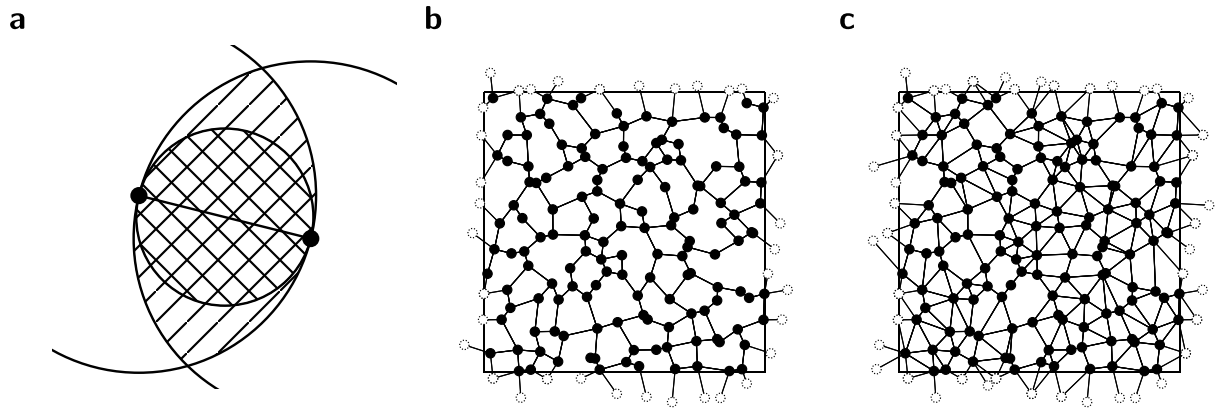
Figure 1. (a) Lunes of two nodes regarding the RNG (hatched region) and GG (cross hatched region), respectively. If there is no node located in the lune, both depicted nodes will be linked by an edge. (b) Example of the RNG with periodic boundary conditions. (c) Example of the GG with periodic boundary conditions. Mirror images of nodes (visualising the periodic boundary conditions) are shown in white.
