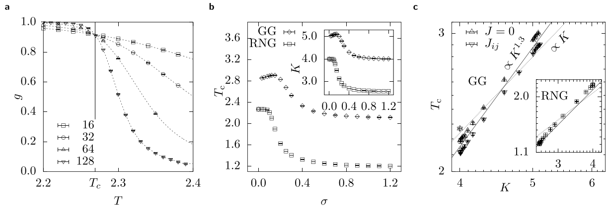
Figure 4. (a) Critical temperatures T_c are obtained by finding the intersections of the Binder cumulants g for different system sizes L . (b) T_c as a function of \sigma . The inset shows the average degree K as a function of \sigma . (c) T_c as a function of K on a log-log scale. The upper curve is for an ensemble where all edges have weight J=1 and the lower curve for length dependent weight J_{ij} . The inset shows the same for the RNG. It is clearly visible that the functional relation T_c(K) is not linear (dotted line) as predicted by the Bethe approximation, but rather a power law T_c \propto K^b with an exponent of b \approx 1.3 (solid line).
