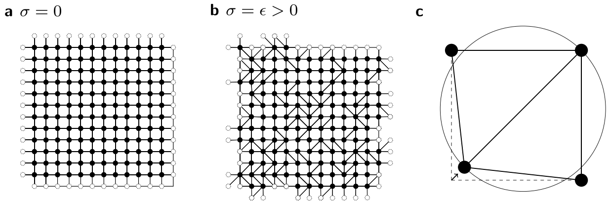
Figure 5. Visualisation of the occurrence of the jump at small values of \sigma for the GG. (a) The regular lattice with no disorder. (b) Example of a graph for a very small value of the disorder. (c) Sketch of a GG with N=4 nodes for very small \sigma . Due to the construction rule of the GG a new edge appears resulting in a jump in K and T_c , see Fig. 4b. This does not occur in the RNG.
