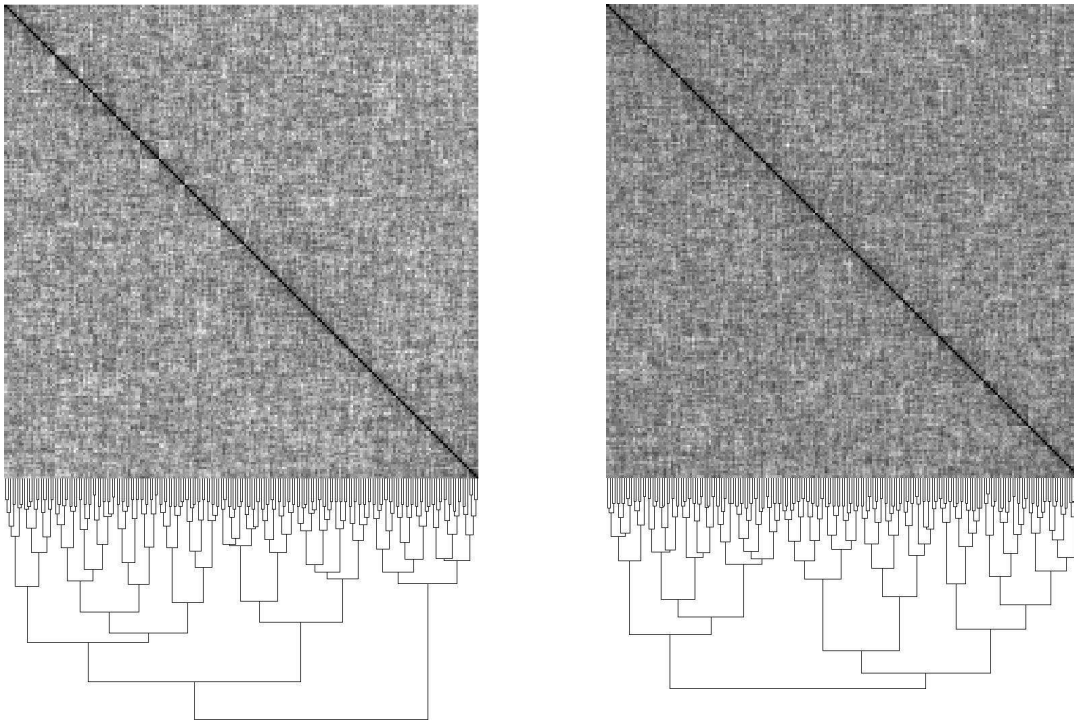
Figure 4. Sample dendrograms (bottom) and distance matrices (top) of 200 NPP solutions for systems with 35 numbers. Darker colors correspond to closer distances. The left one is at k = 1.5 , i. e. in the hard and unsolvable phase, while the right is for k = 0.6 , i.e. in the solvable phase, where perfect partitions exist. In both cases there is no structure present.
