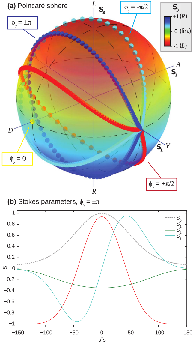
Figure 5. Sampling paths in polarization space, defined by the time-dependent Stokes parameters ( S_1, S_2, S_3 ) and plotted on a Poincaré sphere. (a) Poincaré sphere. Each path on the sphere corresponds to a polarization-shaped pulse created by a spectral phase-step of the type defined in equation (3), as shown in figure 1, with points plotted every 2.5 fs. The paths are parametrized by the Stokes parameters, corresponding to the polarization basis states ( H, V ), ( D, A ) and ( L, R ) respectively [32]. The surface colour-map additionally indicates the S_3 value, hence the pulse polarization in the L/R basis. (b) Time-dependence of the Stokes parameters S_n(t) (here normalized by division by S_0(t) ) for the pulse defined by \phi_y = \pm\pi .
